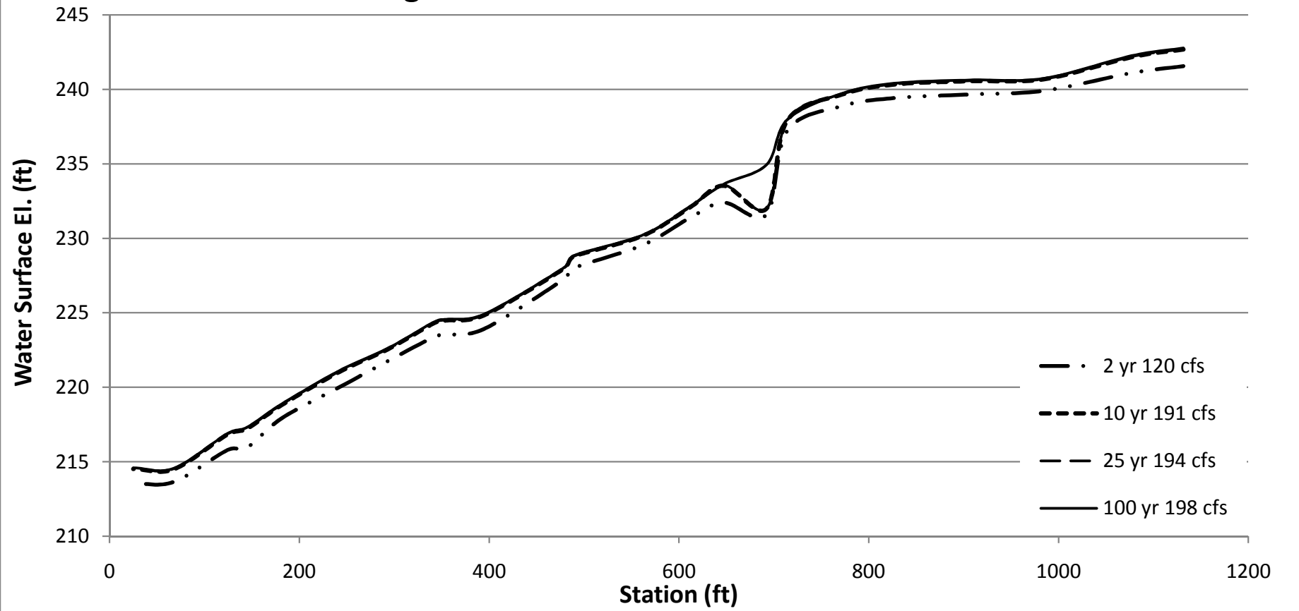
Figure 6. Chimes Creek Flood Profiles
